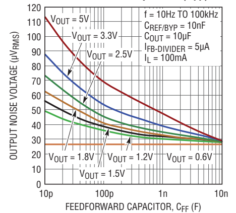
RMS Output Noise vs Feedforward Capacitor ( C_{\text{FF}} )
